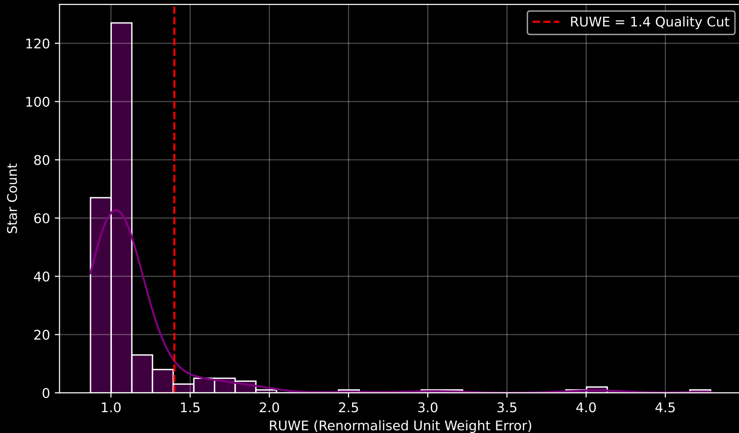
GAPOGEE DR17 Field [N6752] RUWE Distribution (n= 240)
