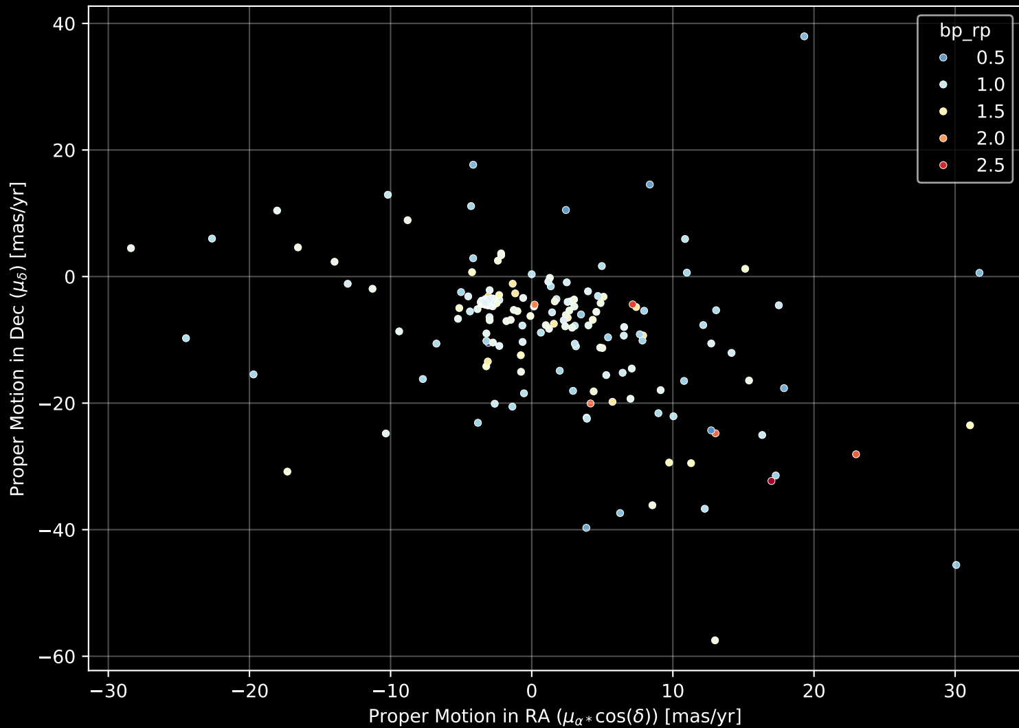
APOGEE DR17 Field: [N6752] Proper Motion Diagram (n= 250)
