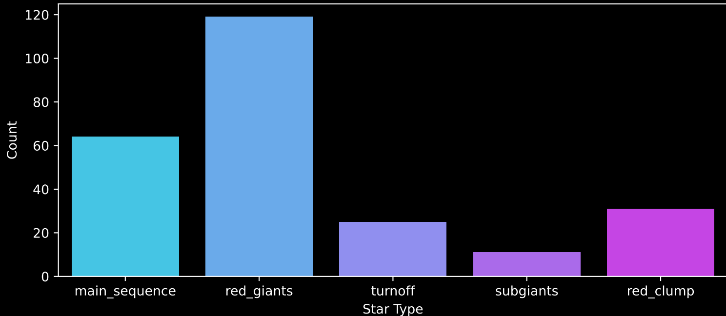
APOGEE DR17 Field: [N6752] Count plot of Star Type
