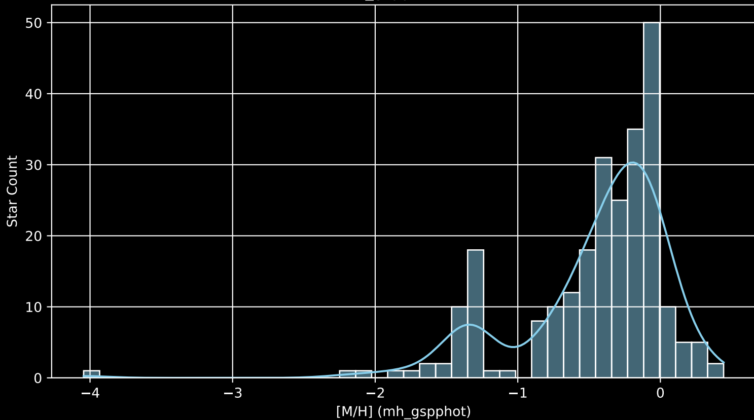
APOGEE DR17 Field: [N6752 [M/H] (mh_gspphot) (n= 250)
