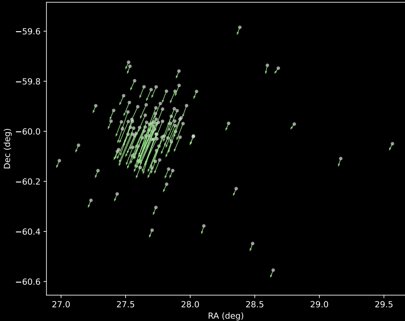
APOGEE DR17 Cluster 5 Proper Motion Vectors (n=109)
