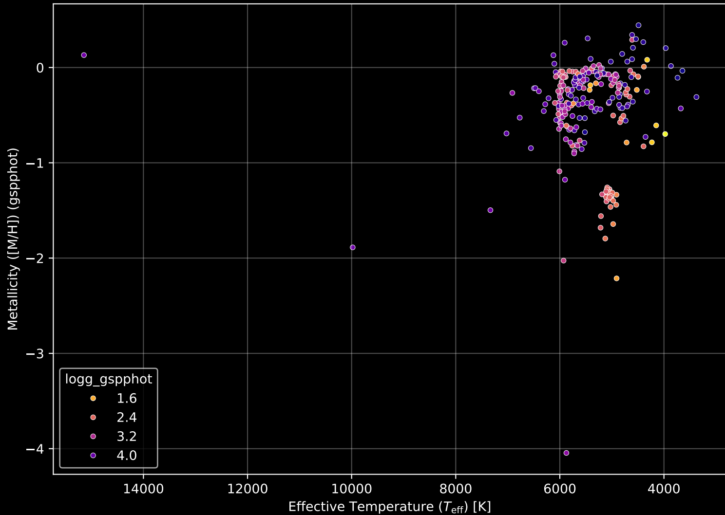
APOGEE DR17 Field: [N6752] Stellar Population Parameters (n= 250)
