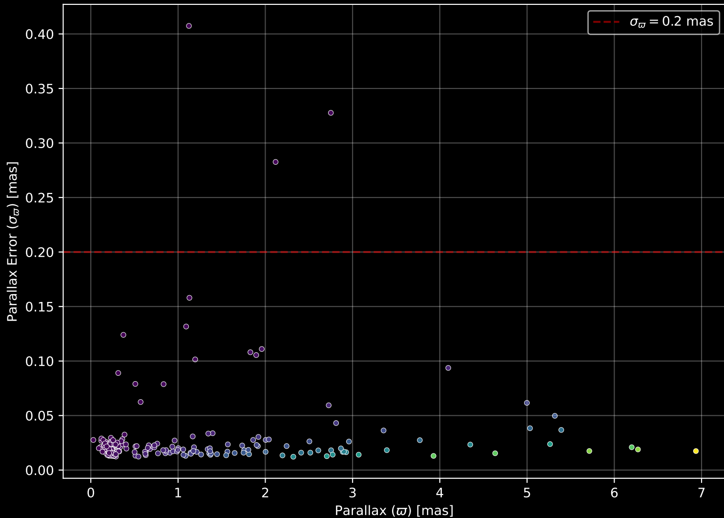
APOGEE DR17 Field: [N6752] Parallax Quality (n= 250)
